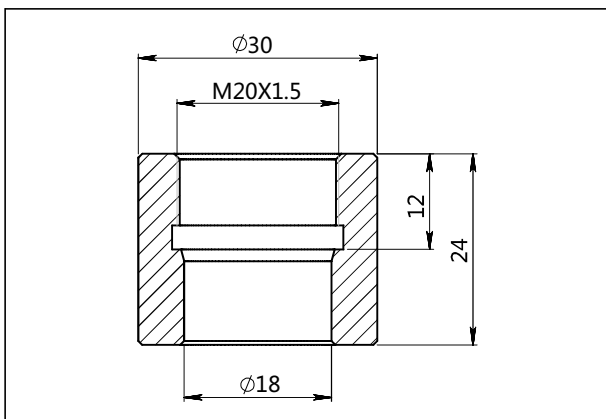
Welding adaptor(Z3)(unit:mm)
