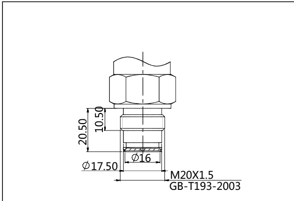
Process connection(G07)(unit:mm)
